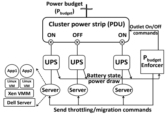
Figure 3. Experimental prototype.
