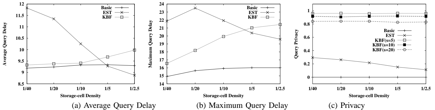
Fig. 11. Comparisons among different schemes
