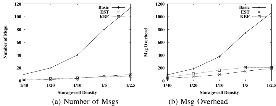
Fig. 10. The message overhead of different schemes
