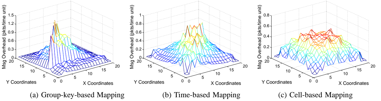
Fig. 4. Message Overhead Distribution of Different Mapping Schemes
