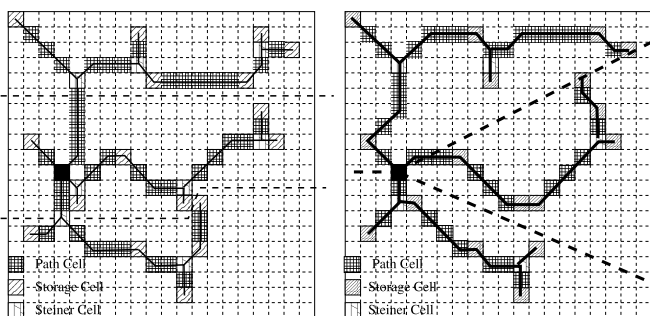
(a) Intuitive partition
