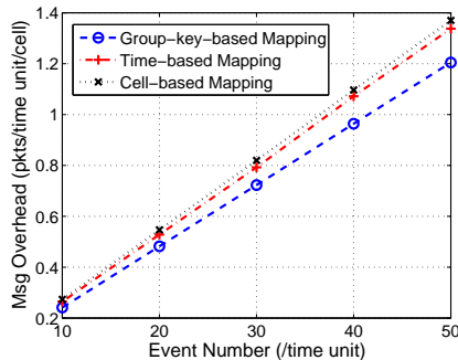
Fig. 3. Overhead Comparisons among different mapping schemes
