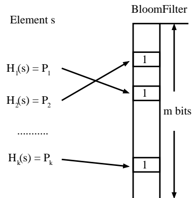
Fig. 7. A Bloom Filter with k hash functions
