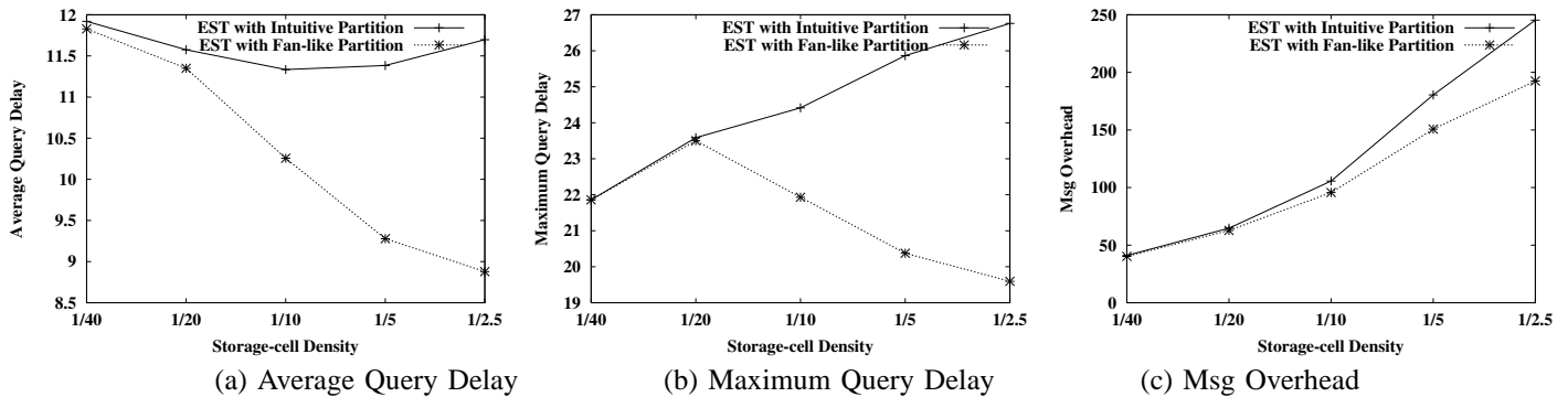
Fig. 9. Performance comparisons between different partitioning schemes
