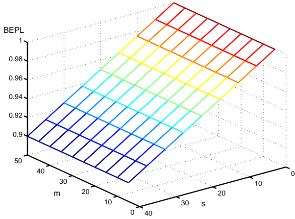
Fig. 2. The BEPL as a function of m and s , where m is the number of detection cells and s the number of compromised cells
