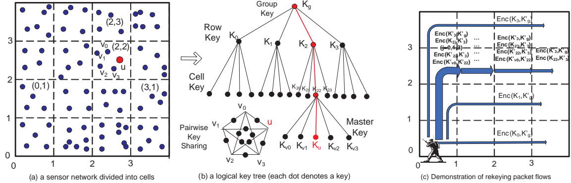
Fig. 5. The mapping between physical network into a logical key tree and the rekeying packet flows for revoking node u
