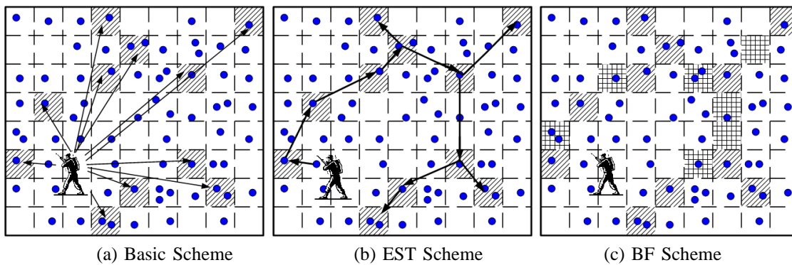
Fig. 6. Three schemes for delivering a query to the storage cells
