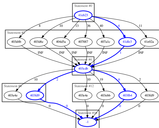
Figure 7: A delta graph instance for an ifelse payload for ngx . The first node is the entry point. Blue nodes and edges form the minimum induced subgraph, H_k . Statement #4 is a conditional, execution branches into two statements. Note that BOPC created this graph.
