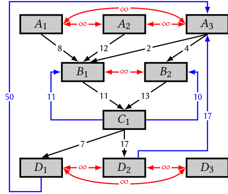
Figure 8: An delta graph instance. The nodes along the black edges form a flat delta graph. In this case, the minimum induced subgraph , H_k is A_3, B_1, C_1, D_1 , with a total weight of 20, which is also the shortest path from A_3 to D_1 . When delta graph is not flat (assume that we add the blue edges), the shortest path nodes constitute an induced subgraph with a total weight of 70. However H_k has total weight 34 and contains A_3, B_2, C_1, D_2 . Finally, the problem of finding the minimum induced subgraph becomes equivalent to finding a k-clique if we add the red edges with \infty cost between all nodes in the same set.
