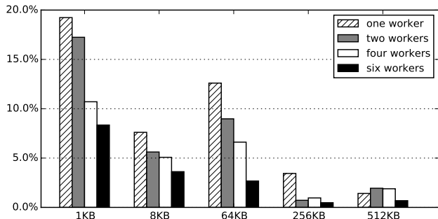
Figure 6: The impacts of different numbers of worker threads on GRIFFIN's performance for the nginx web server.
