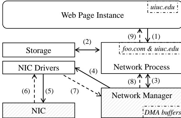
Figure 2: This figure enlarges the right half of Figure 1 and shows how our IBOS subsystems interact when a web page instance from uiuc.edu issues a network request to foo.com . Subsystems are shown in boxes and solid and dotted arrows represent IBOS messages for outgoing and incoming data respectively. The reference monitor (which is not shown here) checks all these messages to enforce security properties.
