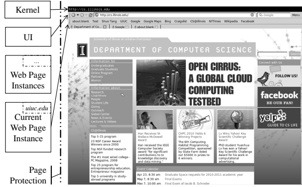
Figure 3: IBOS display isolation. This figure shows how IBOS divides the display into three main parts: a bar at the top for the kernel, a bar for browser chrome, and the rest for displaying web page content. The IBOS kernel enforces this isolation using page protections and without relying on a window manager.
