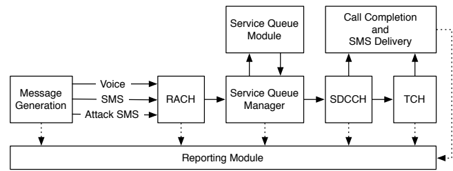
Fig. 24. Simulator Architecture
