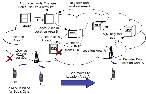
Figure 11: Mixed Identity Attack
