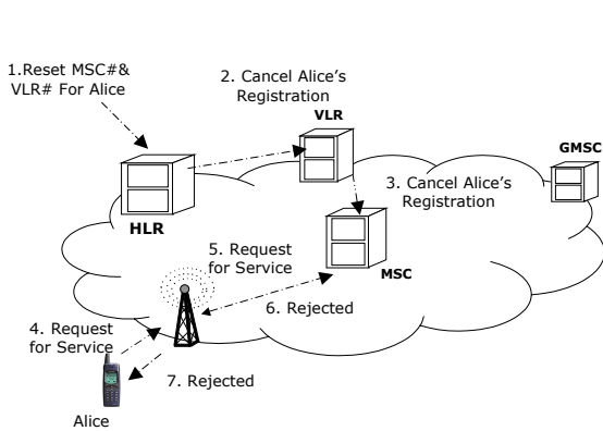
Figure 10: Power Off Power On Attack
