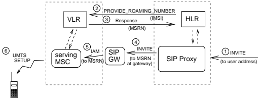
Figure 13: Call setup procedure for proposal 3 — non-IP-enabled visited network
