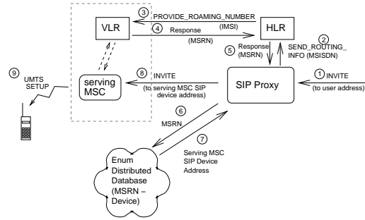
Figure 3: Call setup procedure for proposal 2
