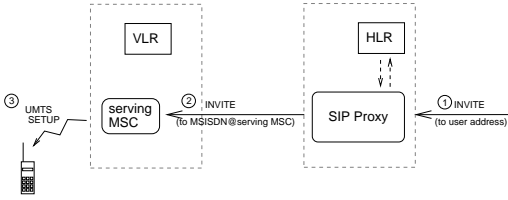
Figure 5: Call setup procedure for proposal 3
