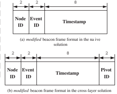
Fig. 4. modified beacon frame format
