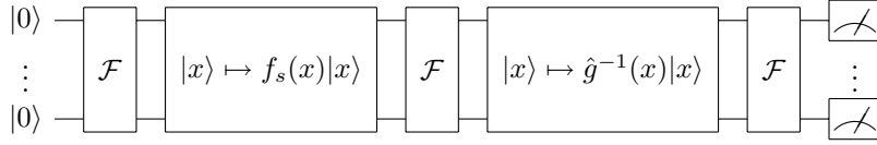
FIG. 3.1. Circuit for hidden shift problem for a known function g and an unknown shift s of the black-box f_s(x) = g(x + s) . Notice that the function values of f_s and \hat{g}^{-1} are computed into the phase.
