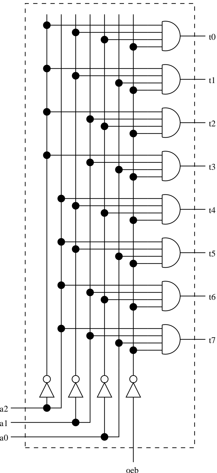
Address Decoder: 3 to 8
