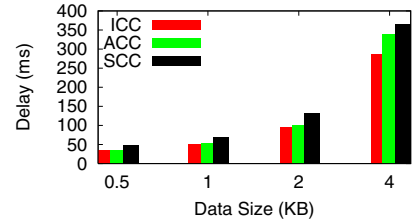
Figure 8. A close view of query latency for different cooperative cache schemes in single-interface-single-channel 802.11 2M ad hoc networks
