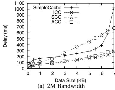
Figure 9. Comparison of the data access delay in wireless mesh networks
