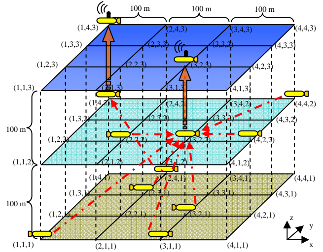
Figure 2. Illustration of the master UUV assignment and data communication schedule involving 10 UUVs on a 4x4x3 grid.
