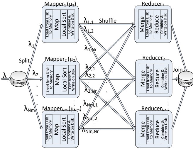
Figure 1. MapReduce framework.
