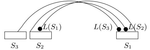
Figure 7: A possible arrangement of sets. Set S_1 is a right set, where as sets S_2 and S_3 are left sets. There are no strong crossings. The right sets form the initial part of the path, while the left sets form the final part.
