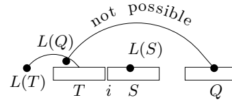
Figure 6: Illustration for the proof of Lemma 5.5. The set S is a straight set, whereas the set T is a right set.
