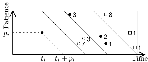
Figure 2: Coordinates of an item i encode t_i & p_i . Each shipment has a capacity of 10. The numbers indicate the weights. The items that are to be shipped together must be enclosed by an angle. Three such shipments are shown.
