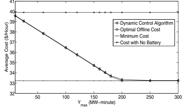
Figure 9: Average Cost per Hour vs. Y_{max} .
