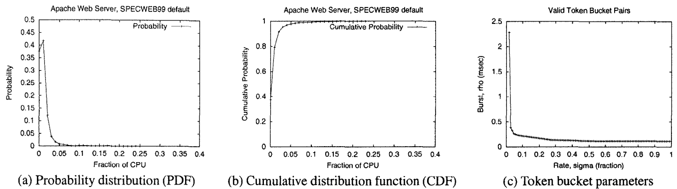
Figure 4: Profile of the Apache web server using the default SPECWeb99 configuration.
