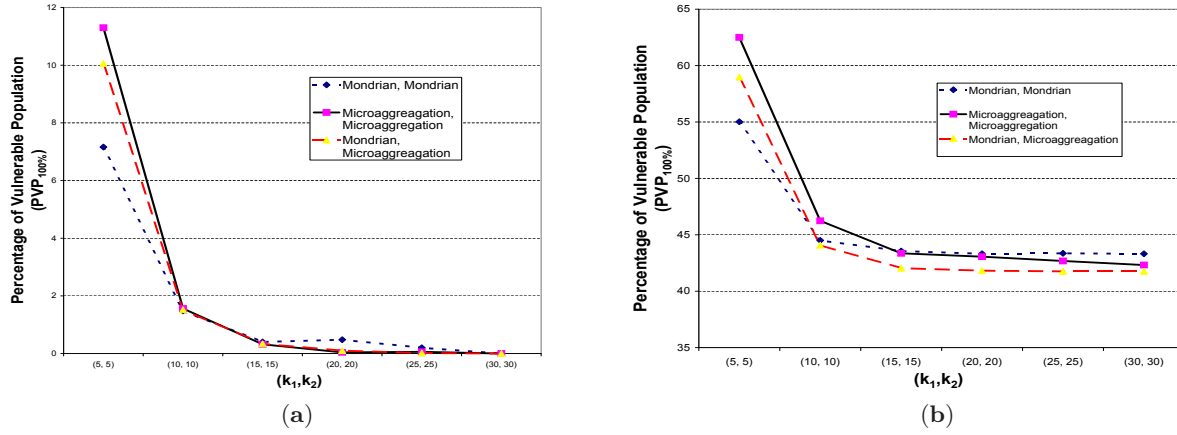
Figure 1: Severity of the intersection attack - perfect breach (a) Adult database (b) IPUMS database.
