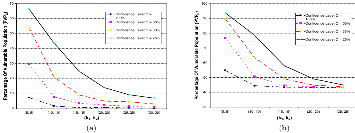
Figure 2: Severity of the intersection attack - partial breach (a) Adult database (b) IPUMS database.
