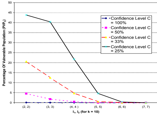
(a) l - diversity
