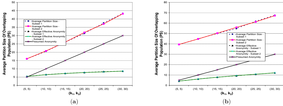
Figure 3: Comparison of presumed anonymity, actual partition sizes, and effective anonymity (a) Adult database (b) IPUMS database.
