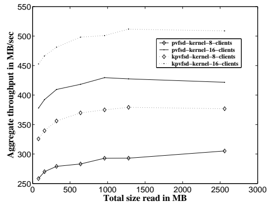
Figure 4. Myrinet: aggregate read bandwidth
