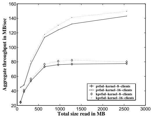
Figure 6. Fast Ethernet: aggregate read bandwidth
