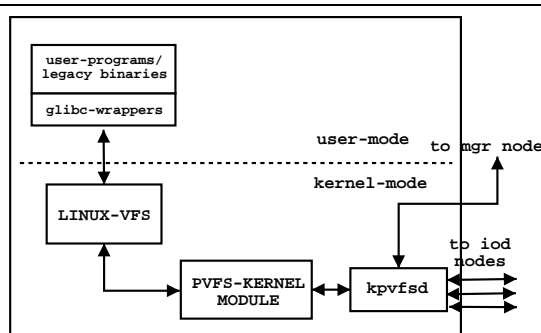
Figure 3. Modified system architecture
