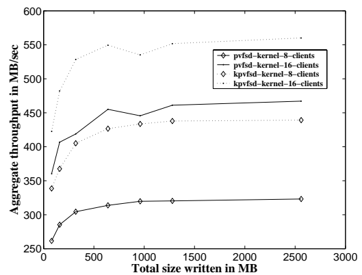
Figure 5. Myrinet: aggregate write bandwidth
