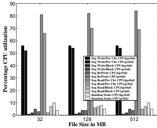
Figure 10. Myrinet: CPU utilization for Bonnie++
