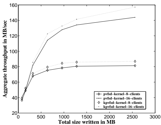
Figure 7. Fast Ethernet: aggregate write bandwidth
