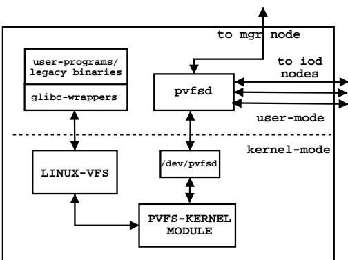
Figure 2. System architecture
