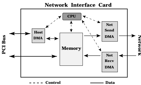
Figure 1. Myrinet NIC
