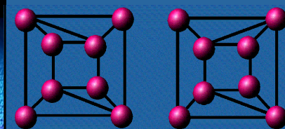
Graph Isomorphism
